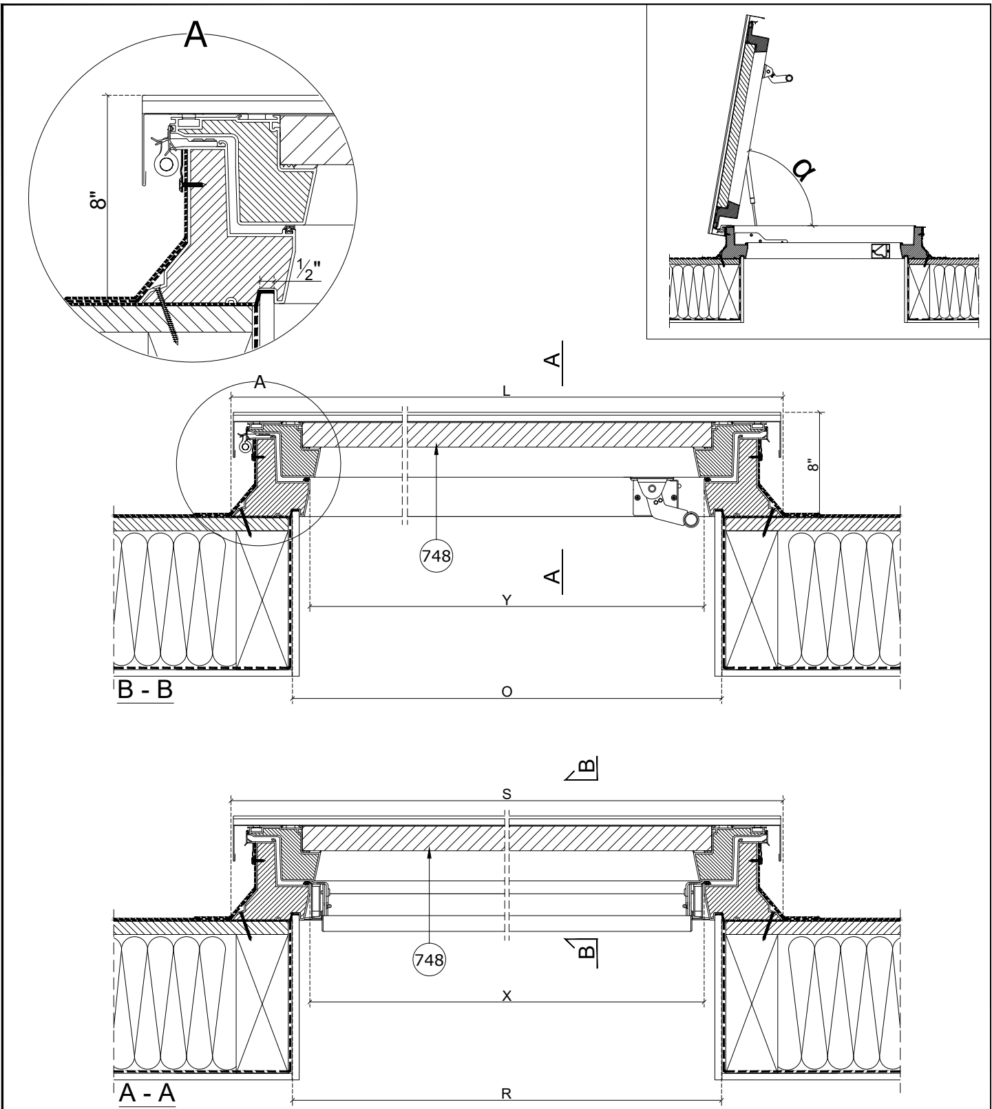
748-DRL FAKRO flat access roof light opened manually
