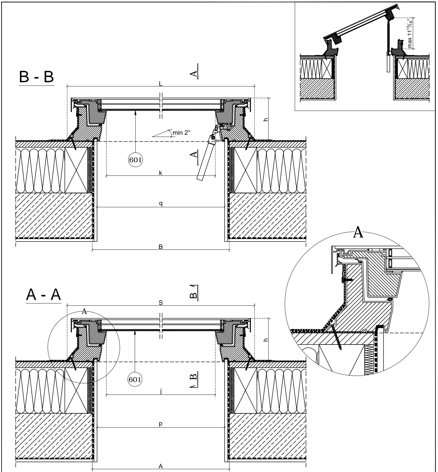
601-DMF DU6 Flat Roof Window, manually opened, Flat, glazing unit DU6
