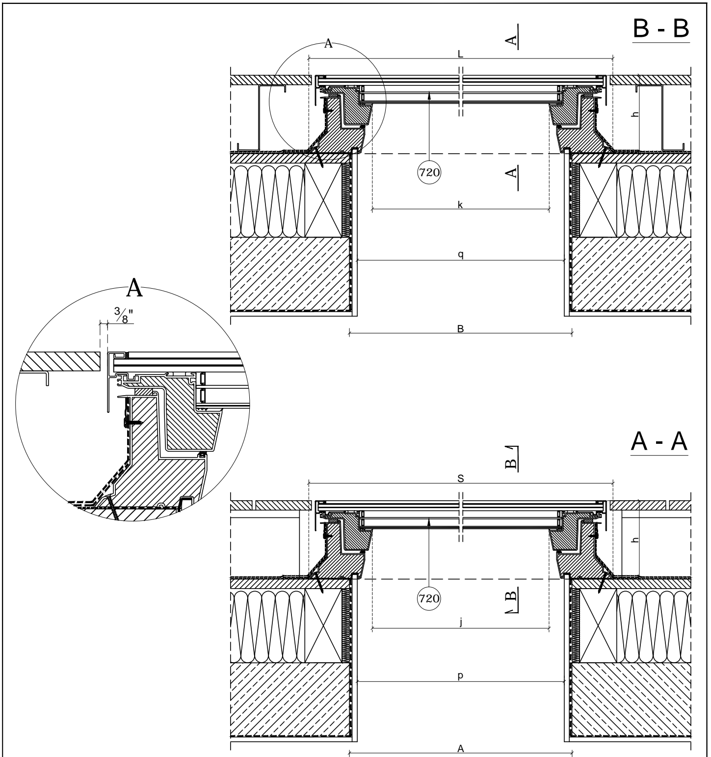
720-DXW DW6 Flat Roof Window, non-opened, Flat, DW6 glazing unit
