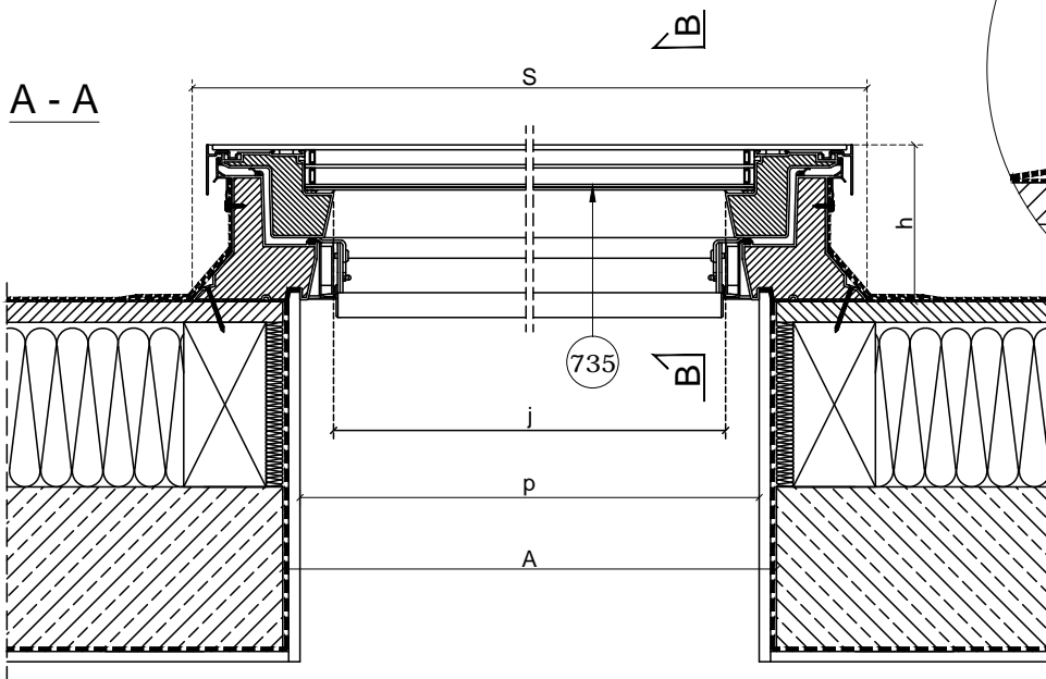
735-DRF DU6 FAKRO flat access roof light opened manually, glazing unit DU6
